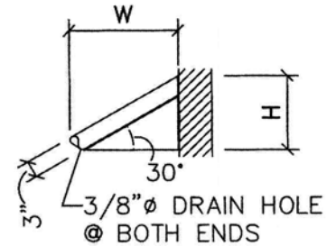
ELEVATION VIEW
