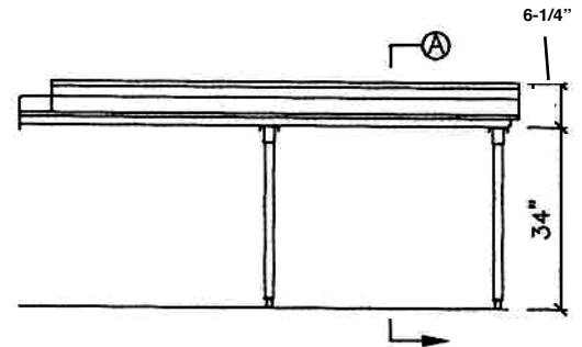
ELEVATION VIEW
