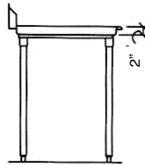
SECTION VIEW
