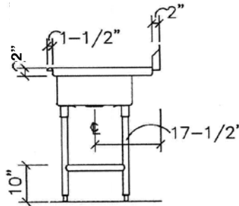
SECTION VIEW
