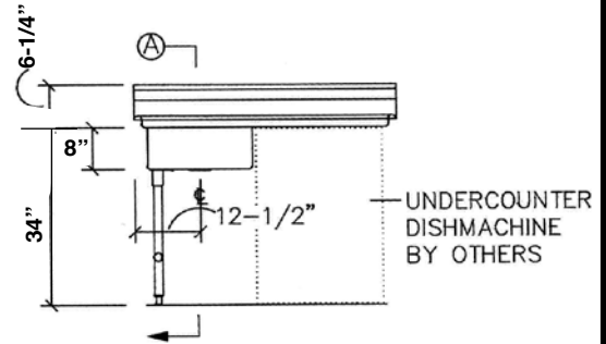
ELEVATION VIEW
