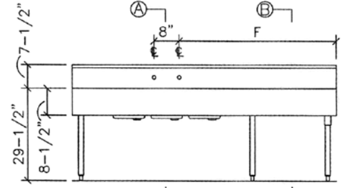
ELEVATION VIEW
