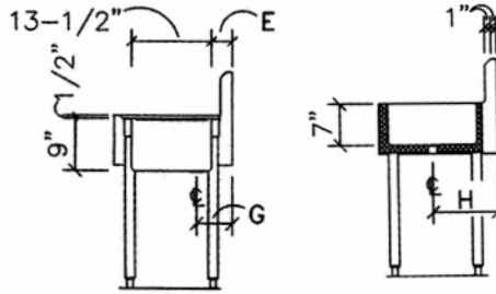
SECTION VIEW
