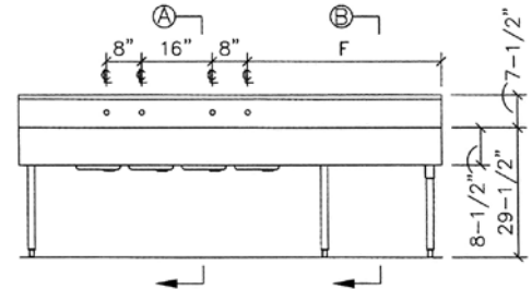
ELEVATION VIEW
