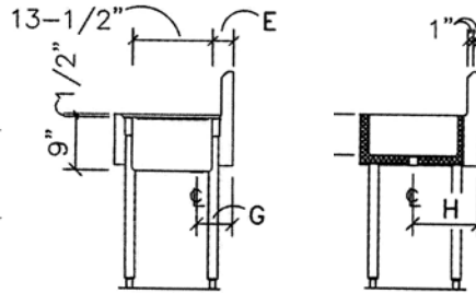
SECTION VIEW
