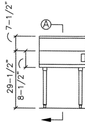
ELEVATION VIEW
