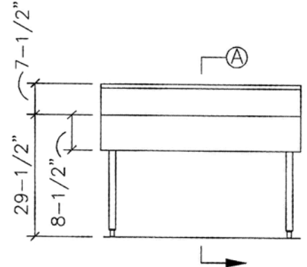
ELEVATION VIEW
