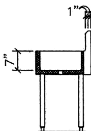
SECTION VIEW
