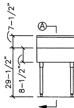
ELEVATION VIEW
