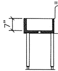
SECTION VIEW
